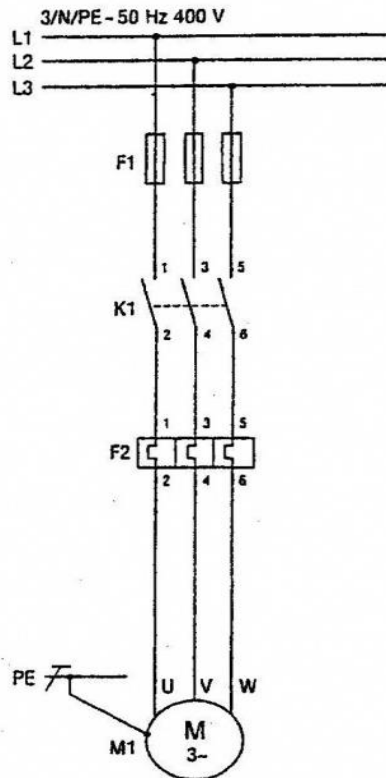
a) Circuito principal
